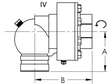
1- 1/2" & 2" Victaulic Type
