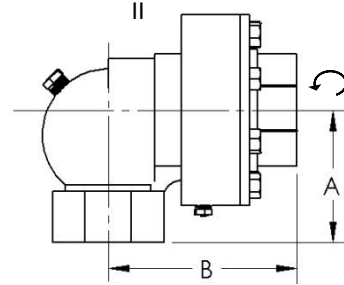
1- 1/2" & 2" Standard Type
