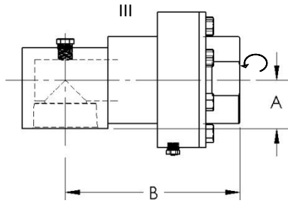
1- 1/2" & 2" Stainless Steel Type
